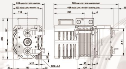
Model : Sicor MR12 Sepehr Lift Co Iran, Isfahan
